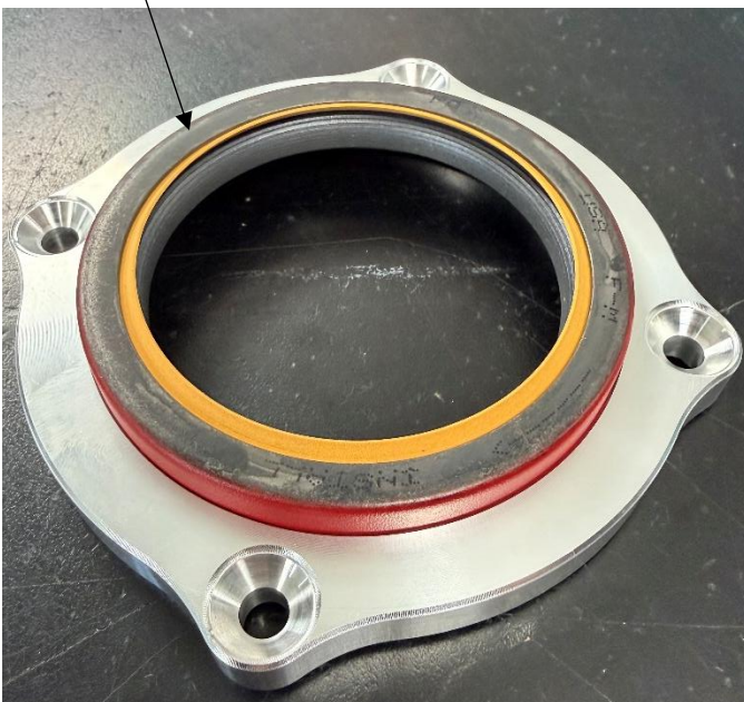
Correct seal orientation
